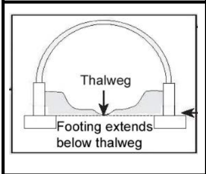
Figure 6-1 Open-bottom culvert
