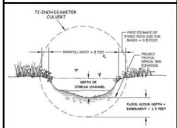
Figure 6-15 Stream simulated culvert cross-section
