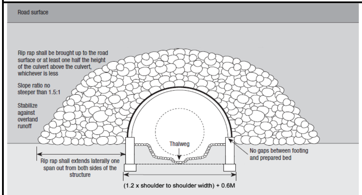
Figure 7-2 Open-bottom culvert – replacement
