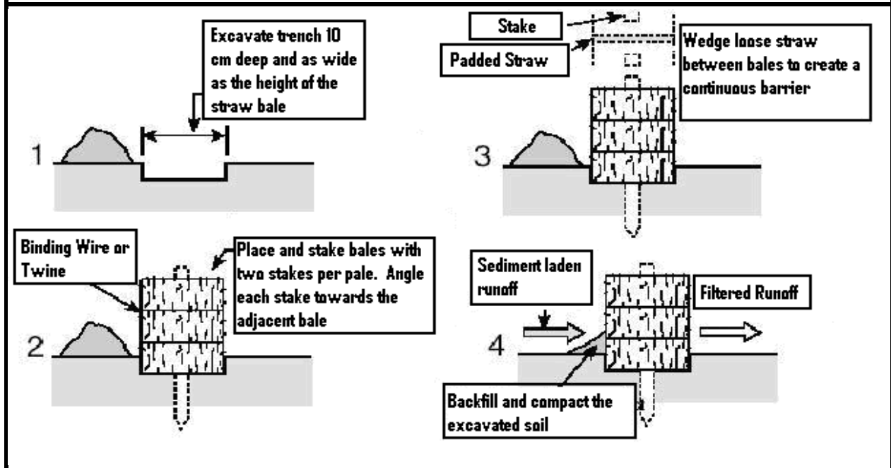
Figure 5-5 Procedure for constructing a straw bale barrier
