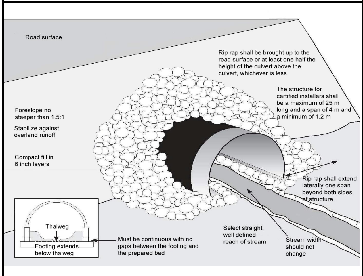
Figure 7-1 Open-bottom culvert – new installation
