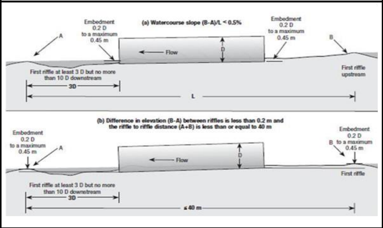
Figure 6-7(a)+(b) Culvert installation when fish baffles are not required
