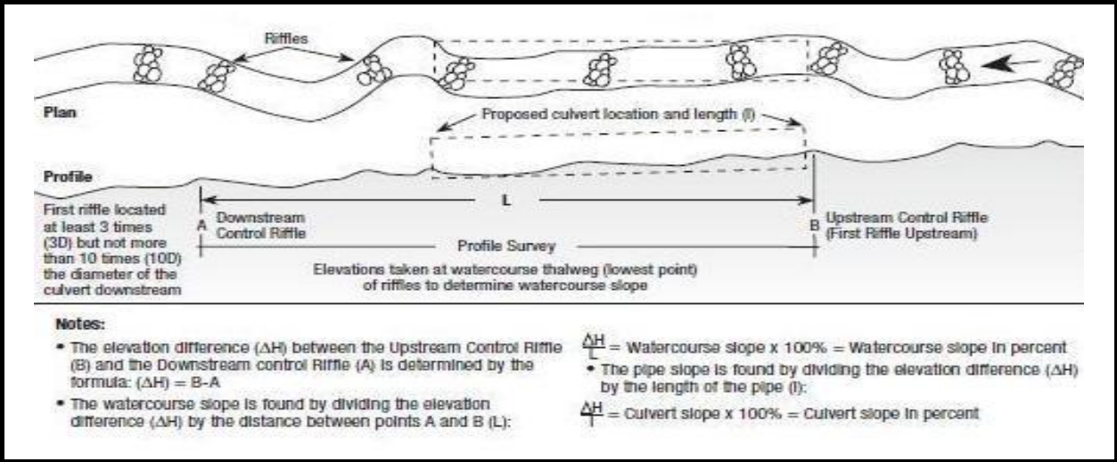
Figure 6-6 Determining the stream gradient
