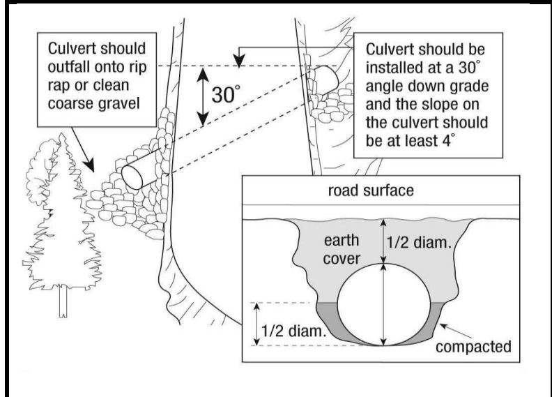
Figure 5-8 Installation of a cross-drainage culvert
