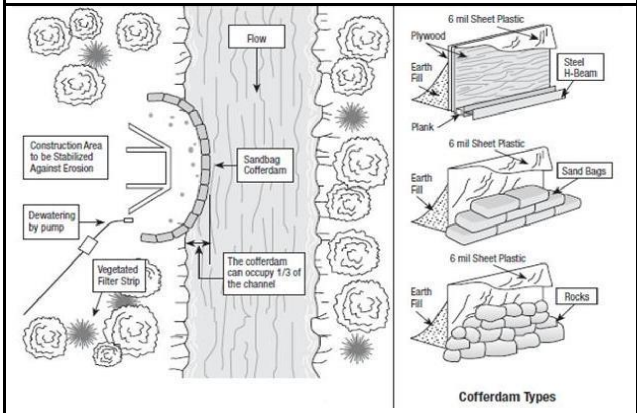
Figure 5-1 A view of a functional cofferdam isolating the construction area and the different types of cofferdams and their components
