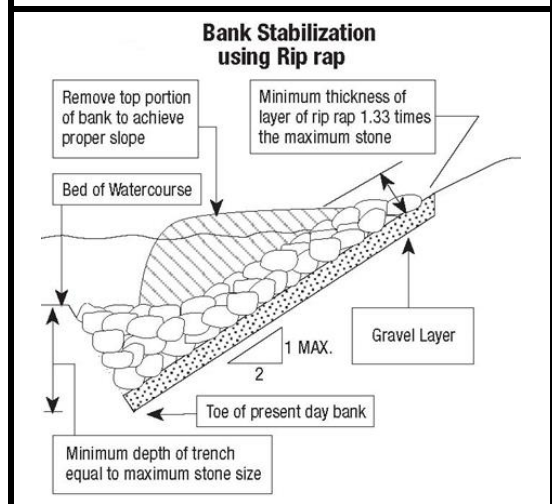
Figure 9-2 Bank stabilization using rip-rap
