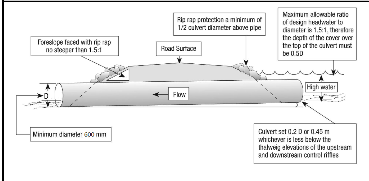
Figure 6-11 Guidelines required for culvert installation
