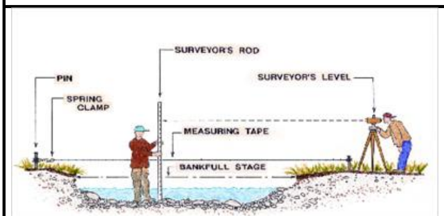
Figure 4-1 Measuring the cross-section of a channel
