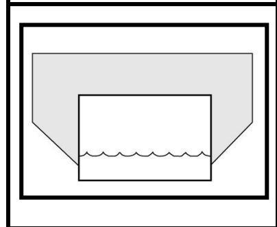
Figure 6-2 Box culvert
