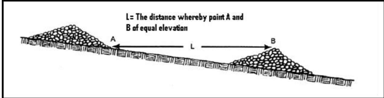
Figure 5-4 Measuring the placement of check dam distance
