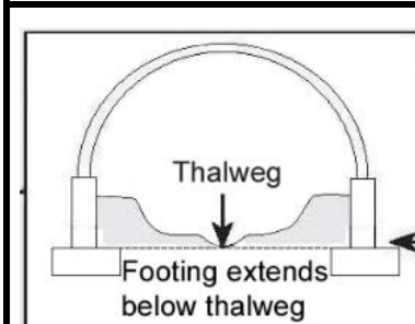
Figure 7-1 Open-bottom culvert
