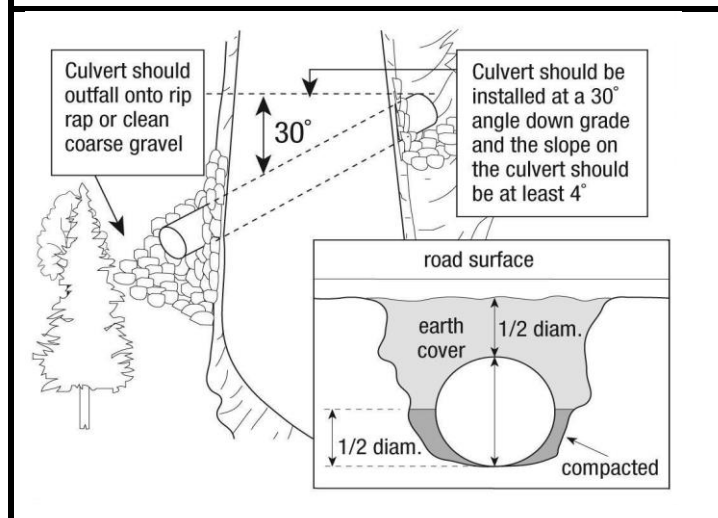
Figure 6-8 Installation of a cross-drainage culvert
