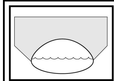
Figure 7-3 Pipe arch culvert
