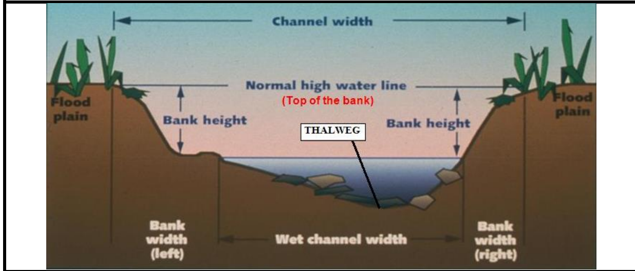
Figure 4-3 Watercourse characteristics (cross-section view)
