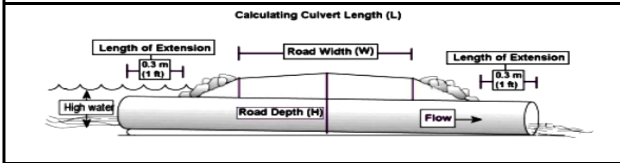
Figure 7-14 Parameters for calculating culvert length
