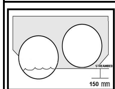
Figure 7-4 Multiple culvert
