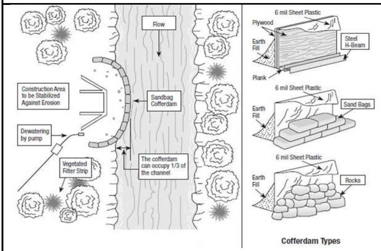
Figure 6-1 A view of a functional cofferdam isolating the construction area and the different types of cofferdams and their components
