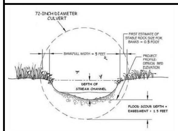
Figure 7-21 Stream simulated culvert cross-section
